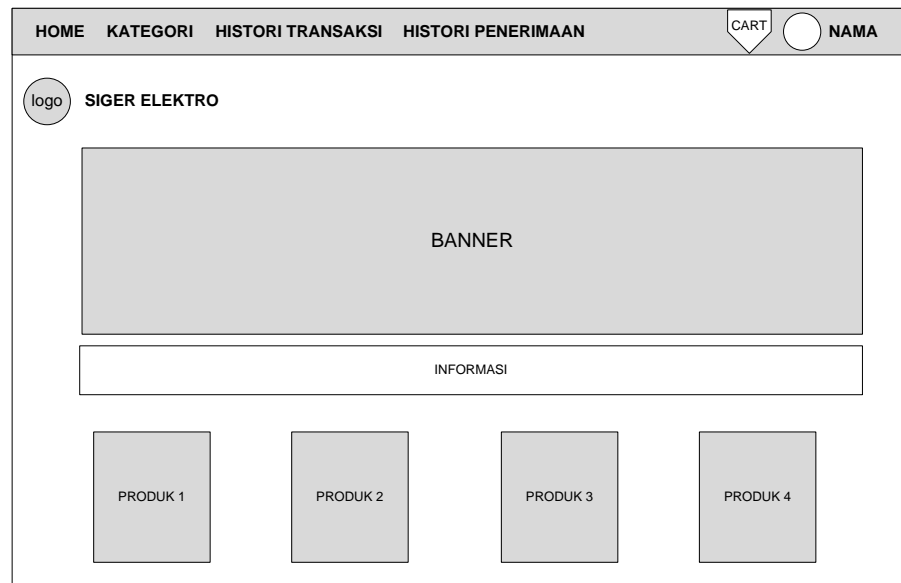
Gambar 4.11 Halaman Customer
