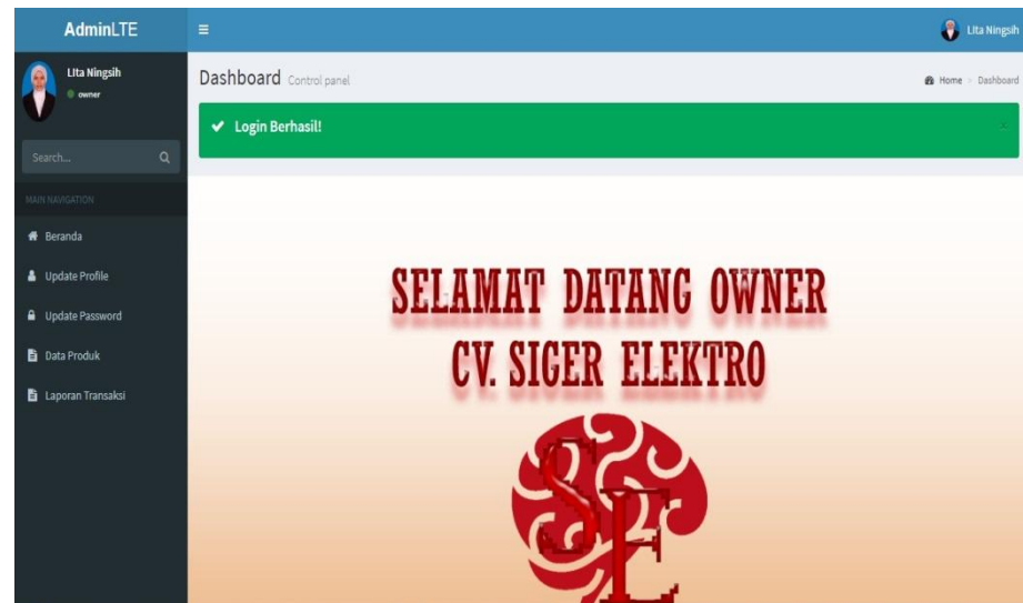
Gambar 4.41 Halaman Owner
