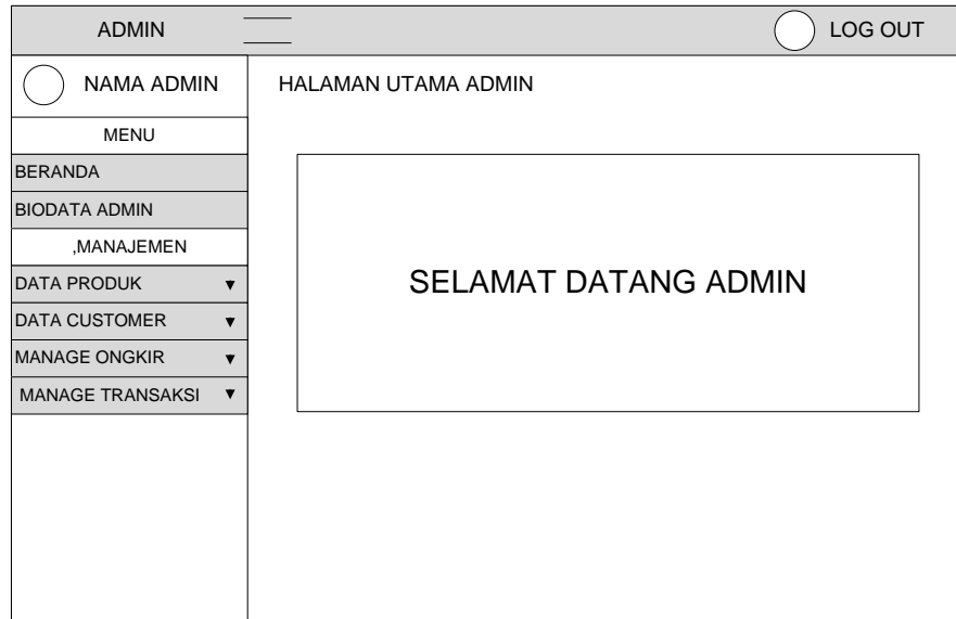
Gambar 4.9 Halaman Admin
