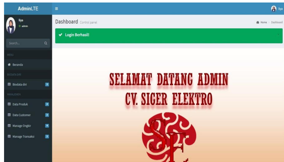
Gambar 4.42 Halaman Admin
