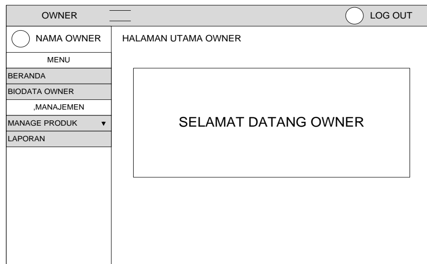
Gambar 4.10 Halaman Owner
