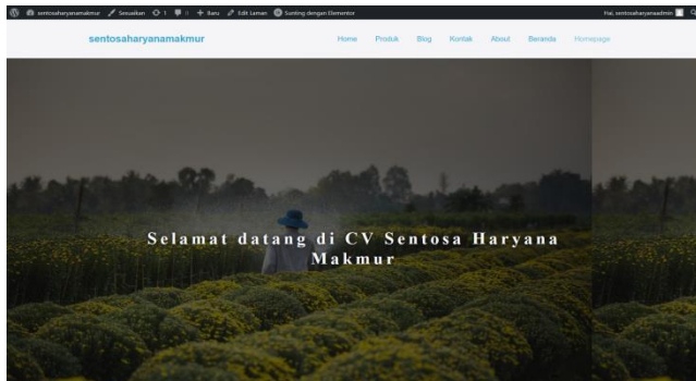
Gambar 2.1 Halaman Website
