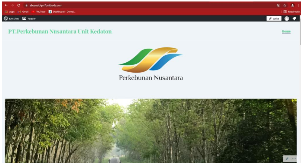
Gambar 4.8 Tampilan Home
