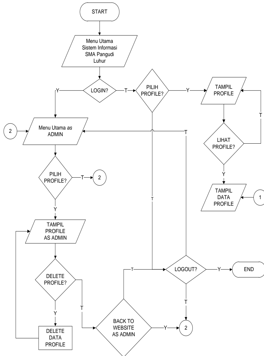
.Gambar 4.34 Flowchart Program Menu Profile
