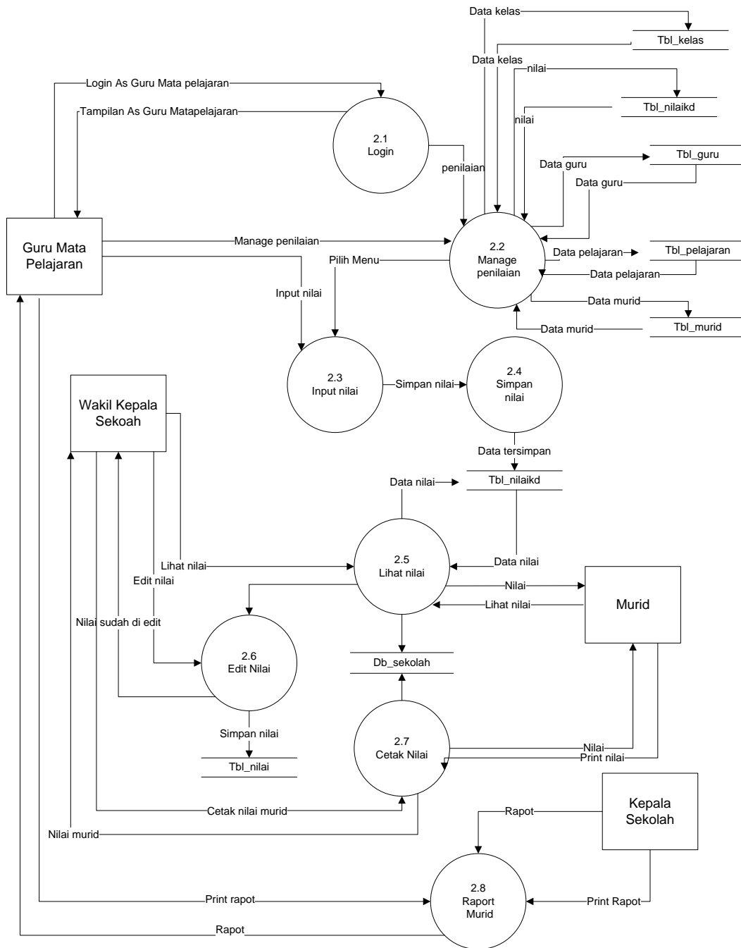
Gambar 4.6 DFD Level 1 Proses 2 Sub Sistem Penilaian.
