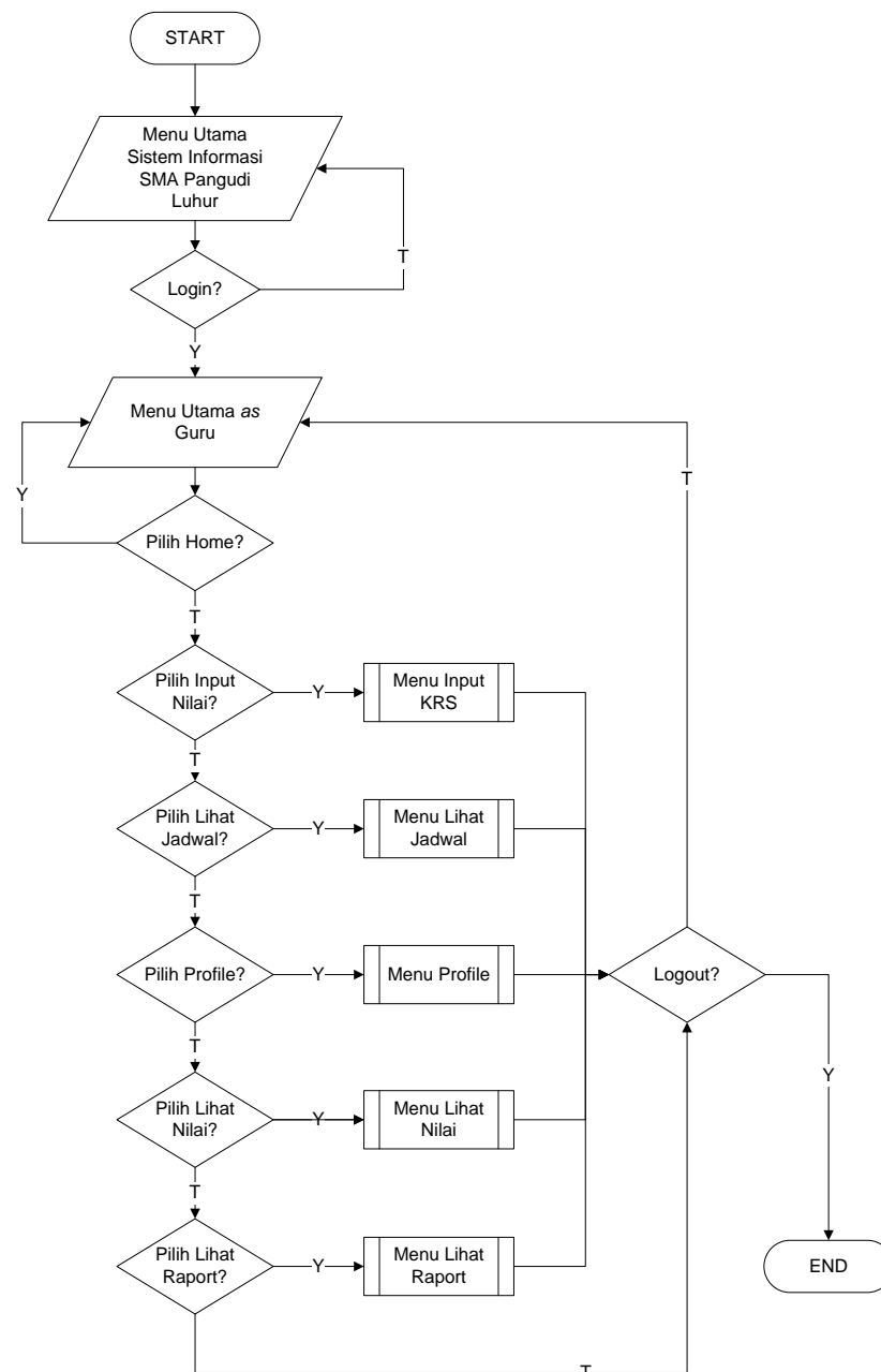
Gambar 4.30 Flowchart Program Guru
