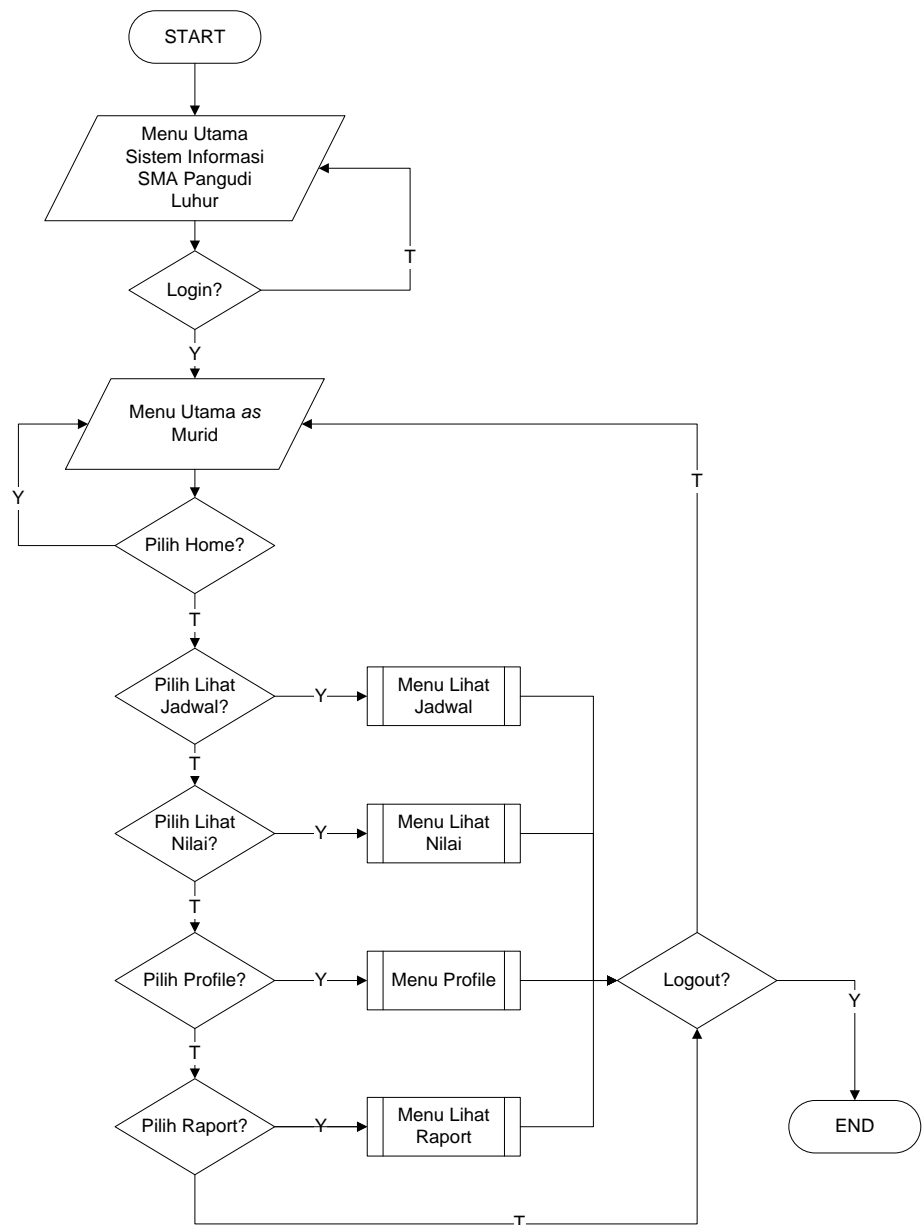
.Gambar 4.31 Flowchart Program Murid
