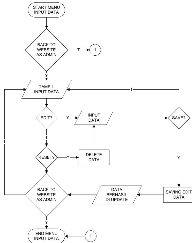
.Gambar 4.32 Flowchart Program Input Data
