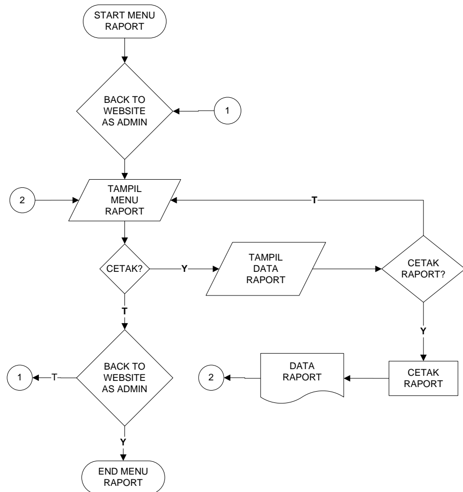
Gambar 4.37 Flowchart Program Menu Raport
