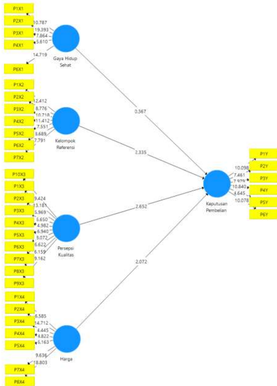
Boostrapping Model
