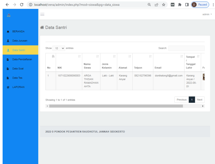
Gambar 4.4 Tampilan halaman Data Santri
