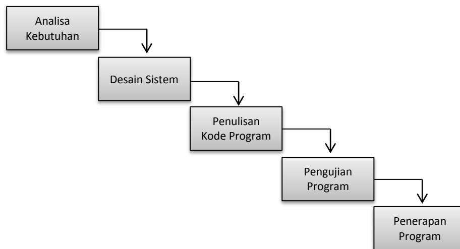
Gambar 2.1 Metode Waterfall
