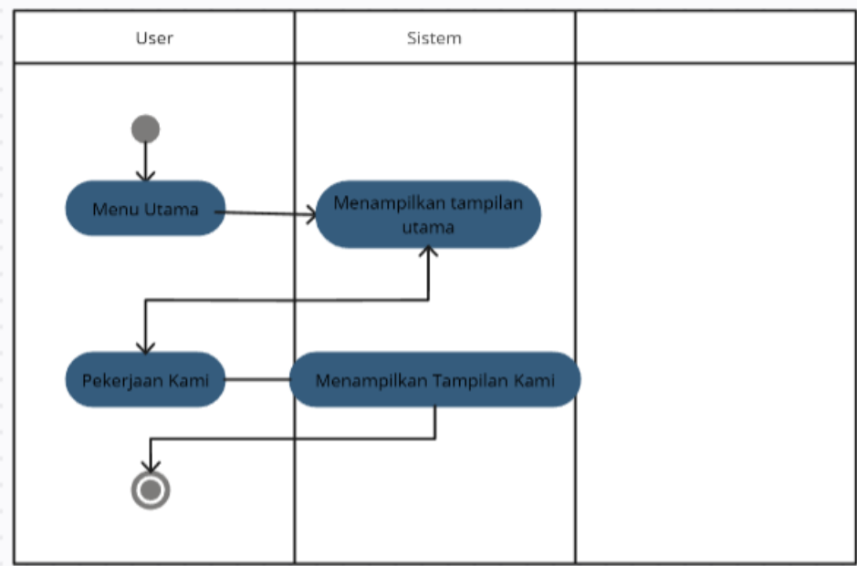
Gambar 2.4 Activity Diagram Pekerjaan Kami
