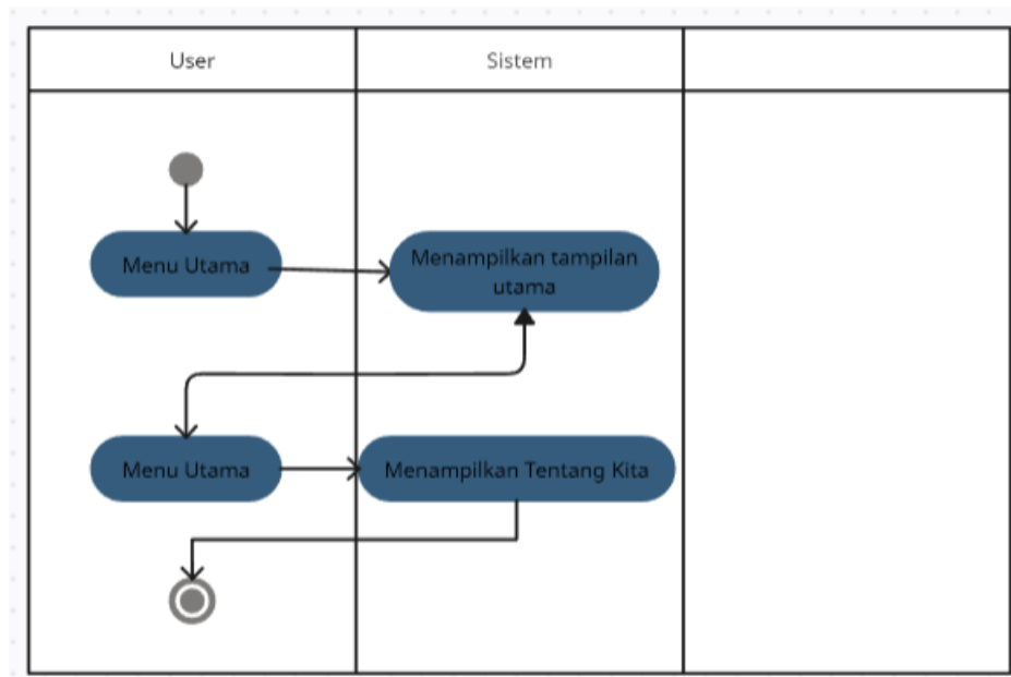
Gambar 2.2 Activity Diagram Tentang Kita
