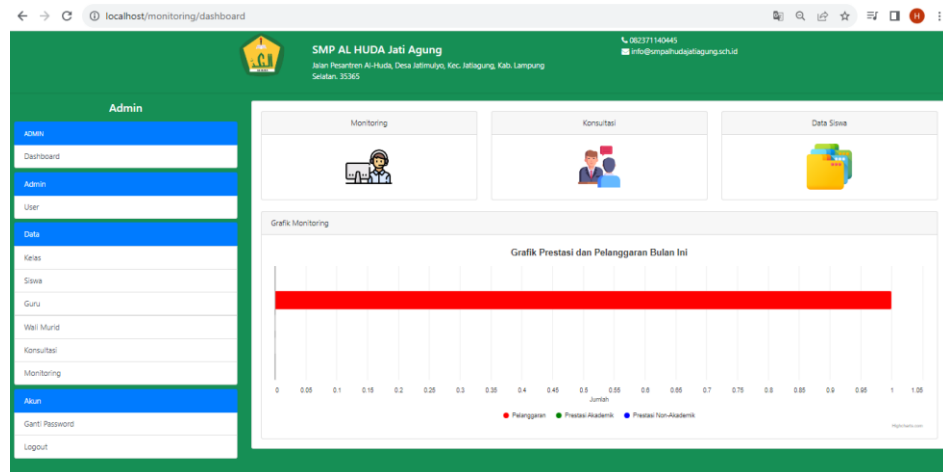
Gambar 4.2 Menu Dashboard.
