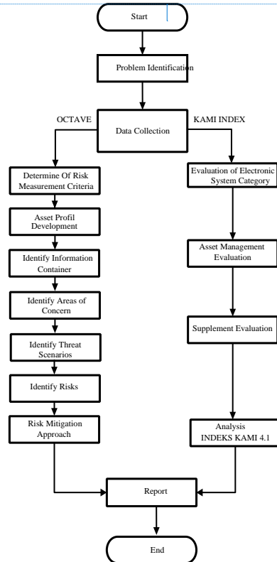
Figure 2. Research flowchart
