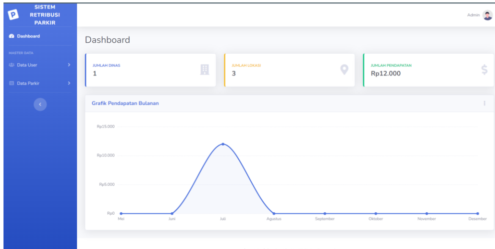
Gambar 4.18 Halaman Dashboard
