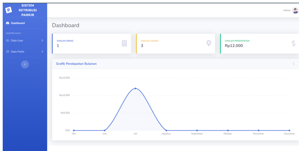
Gambar 4.2 Halaman Dashboard
