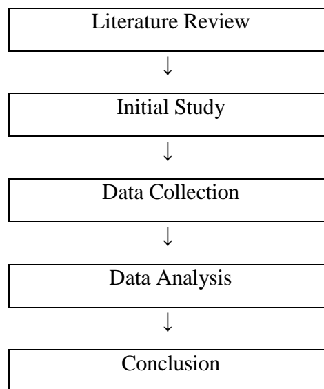
Figure 1. Research Method
