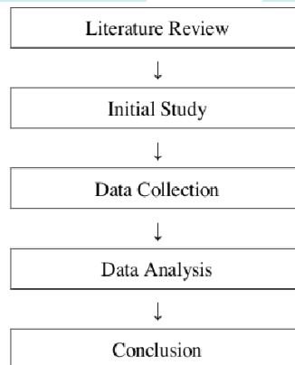
Figure 1. Research Method
