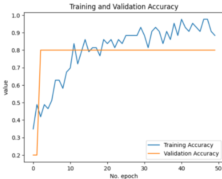
Gambar 3. 2 Visualisasi data Training Accuracy dan Validarion Accuracy
