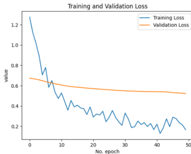
Gambar 3. 1 Visualisasi data Training Loss dan Validation Loss
