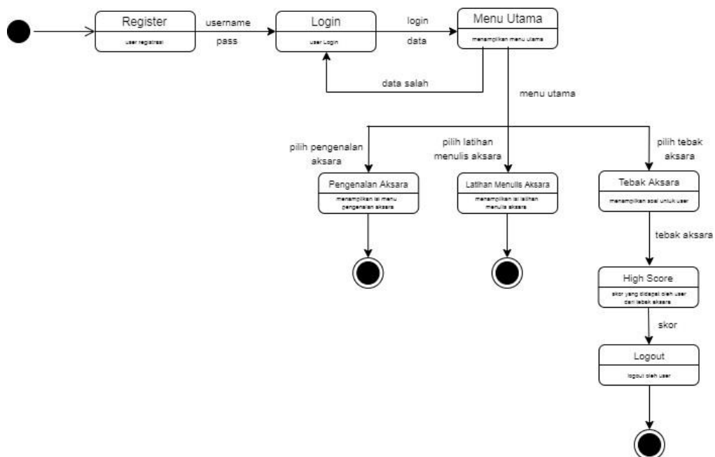
Gambar 3.16 State Diagram
