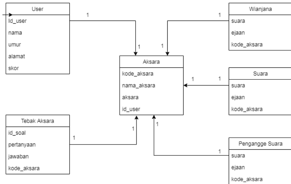
Gambar 3.15 Class Diagram
