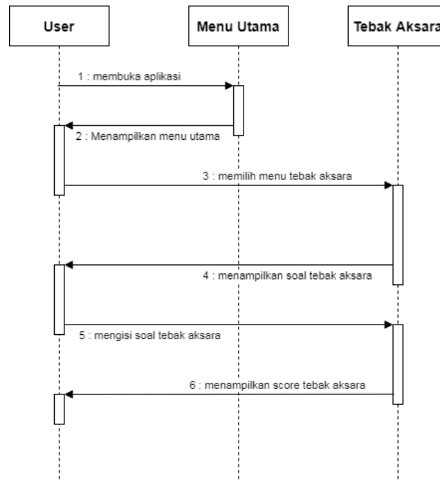
Gambar 3.12 Sequence Diagram Tebak Aksara
