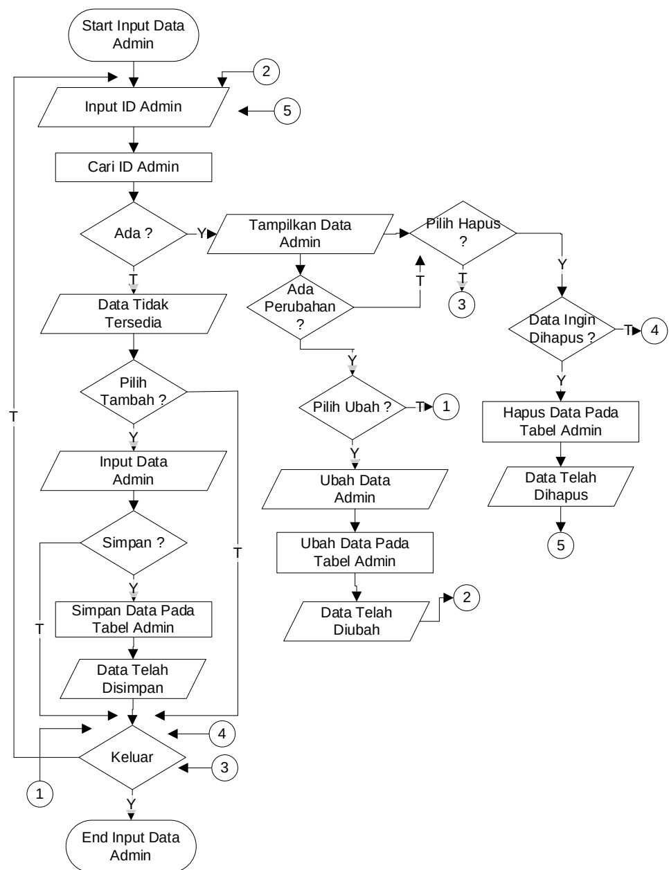
Gambar 4. 11 Flowchart form data Admin
