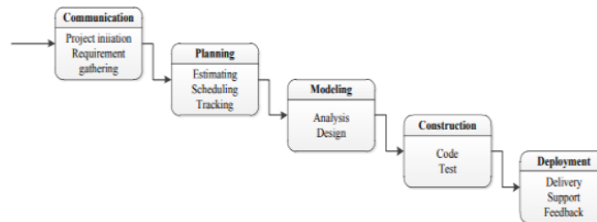
Gambar 1. Model Waterfall (Pressman, 2015).
