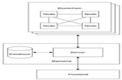
Figure 7. Blockchain E-Voting Architecture.
