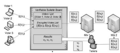
Figure 5: A typical re-encryption mix-net
