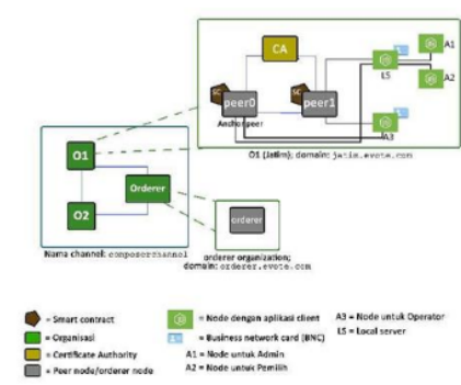
Figure 8. Organizational design in the scope of blockchain
