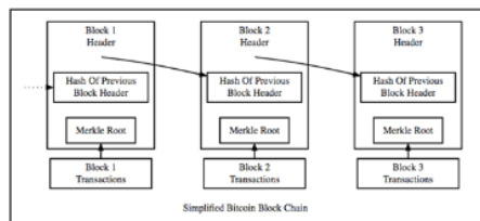
Figure 2: Blockchain transaction structure.2
