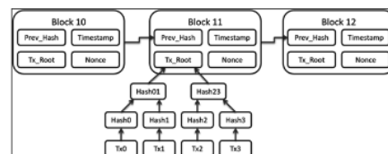
Figure 3: Information stored in each block.
