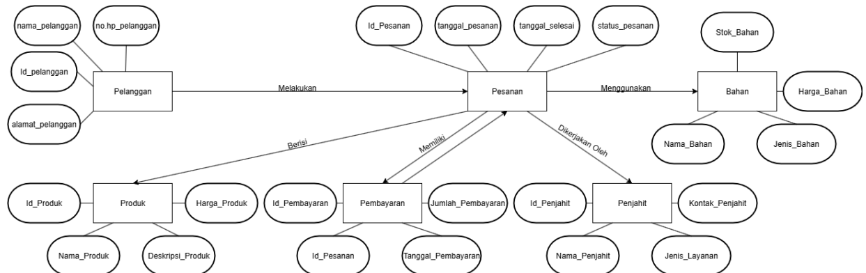
Gambar 2.2 ERD Perancangan Website Ria Jahit
