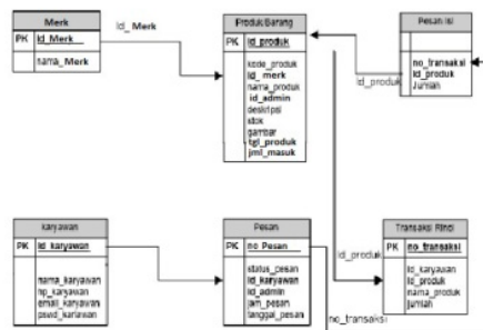
Gambar 7 LRS sistem informasi riwayat receiver
