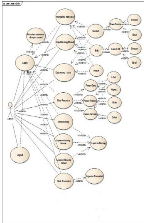
Gambar 2 Use Case Admin
