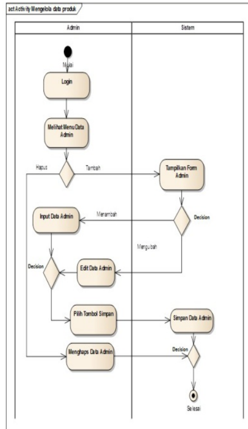
Gambar 4. Activity Diagram Data Admin
