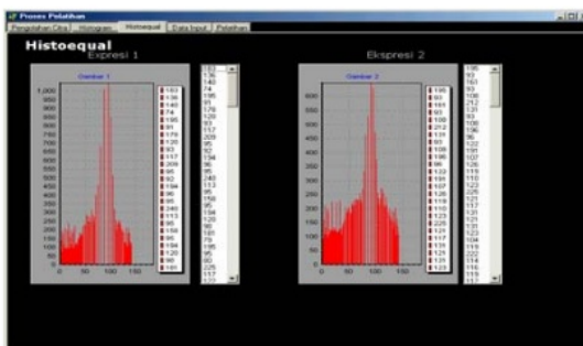
Gambar 4.2 Histoqual
