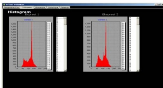
Gambar 4.1 Histogram
