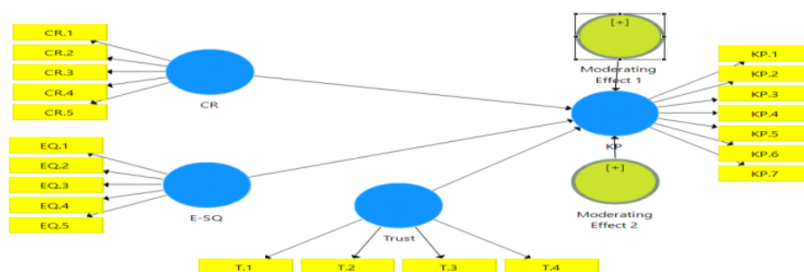
Gambar 3. Skema Model Partial Least Square (PLS)
