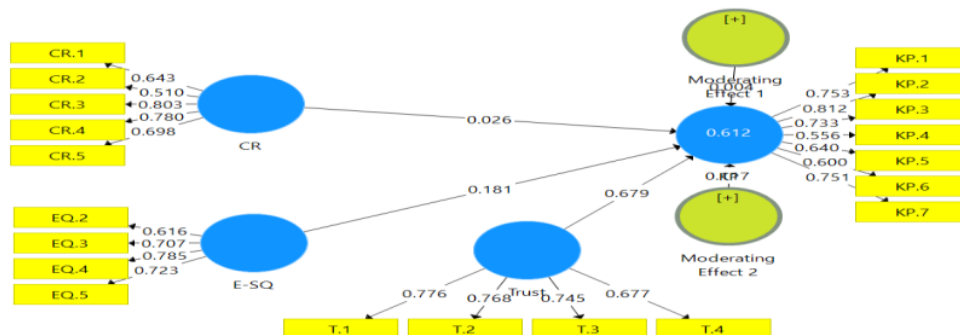
Gambar 4. Outer Model (PLS-SEM Algorithm)
