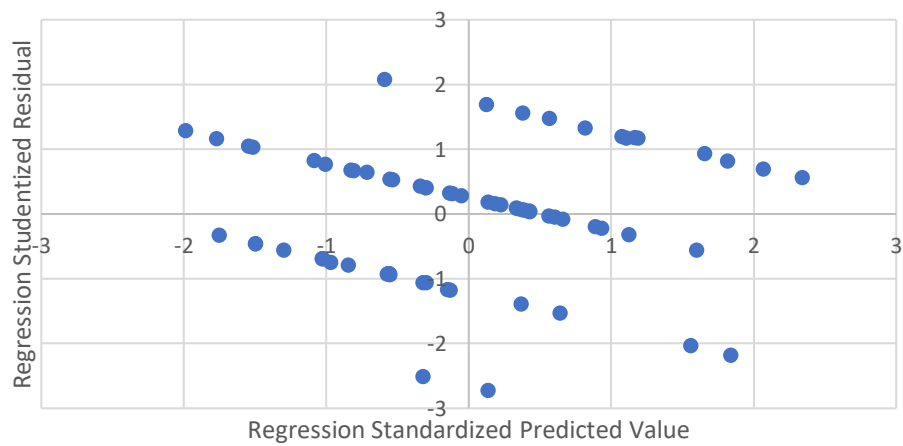
Scatterplot
