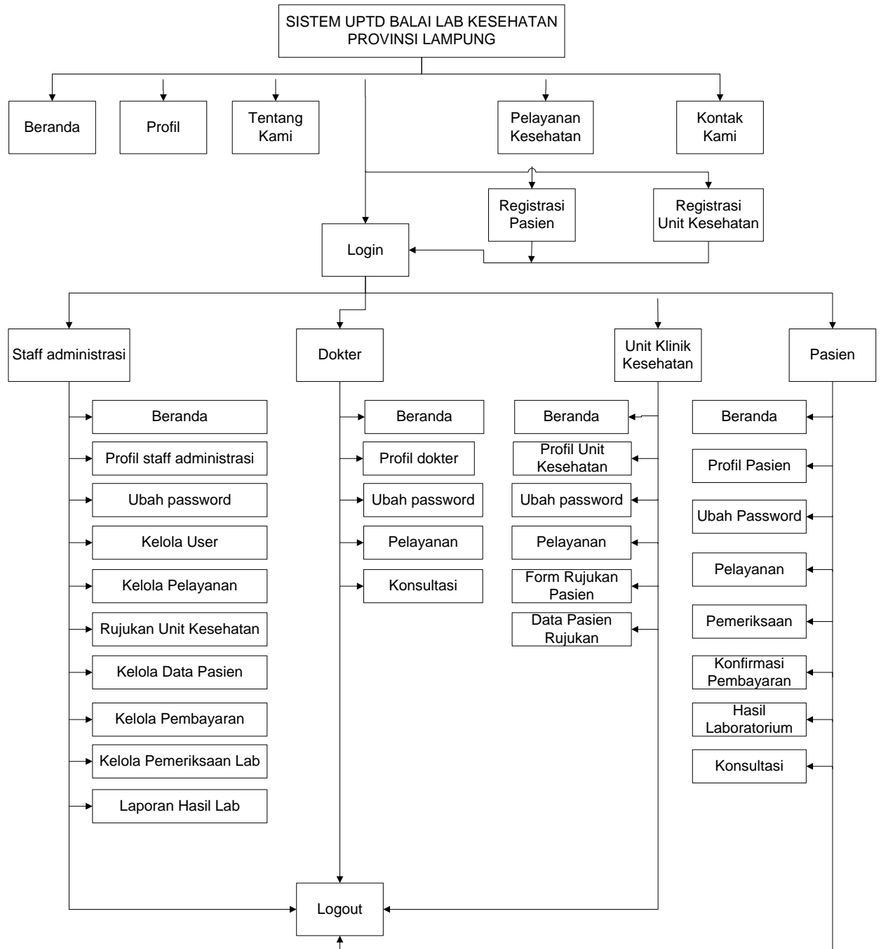
Gambar 4.1 Hierarchy Plus Input-Proses-Output (HIPO) .
