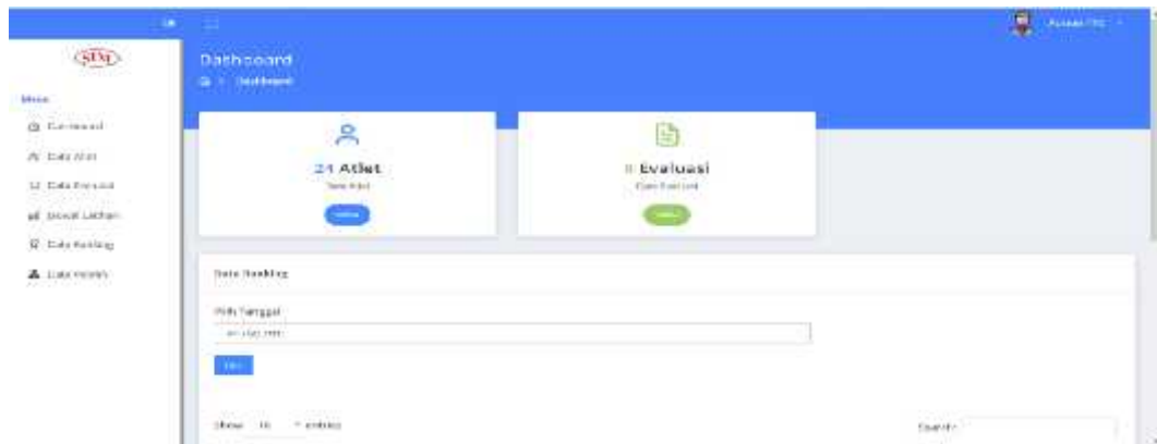
Gambar 4.2 Tampilan Dashboard
