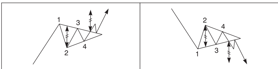
Figure 7.3 Triangles
