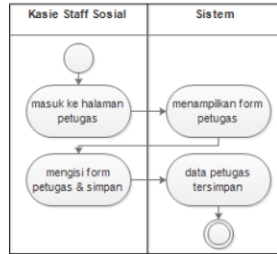
Gambar 7. Perancangan Activity Diagram Mengolah Data Staff
