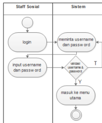
Gambar 4 Perancangan Activity Diagram Login
