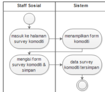
Gambar 5 Perancangan Activity Diagram Input Data
