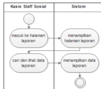
Gambar 8. Perancangan Activity Diagram Laporan Hasil Survey
