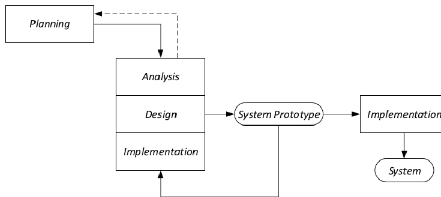
Gambar 1. Prototyping-Based Methodology
