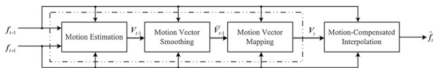
Fig. 2 Framework of MC-FRUC
