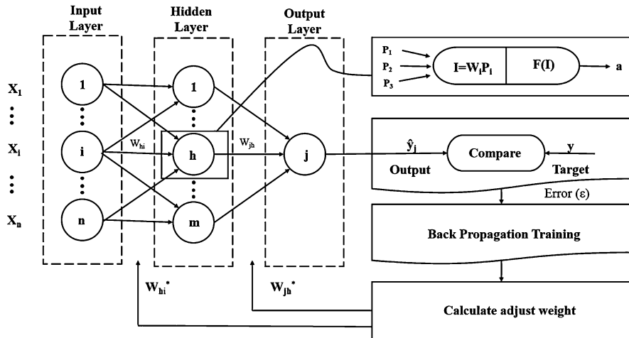
Fig. 1 Schematic of a three layer FFNN model
