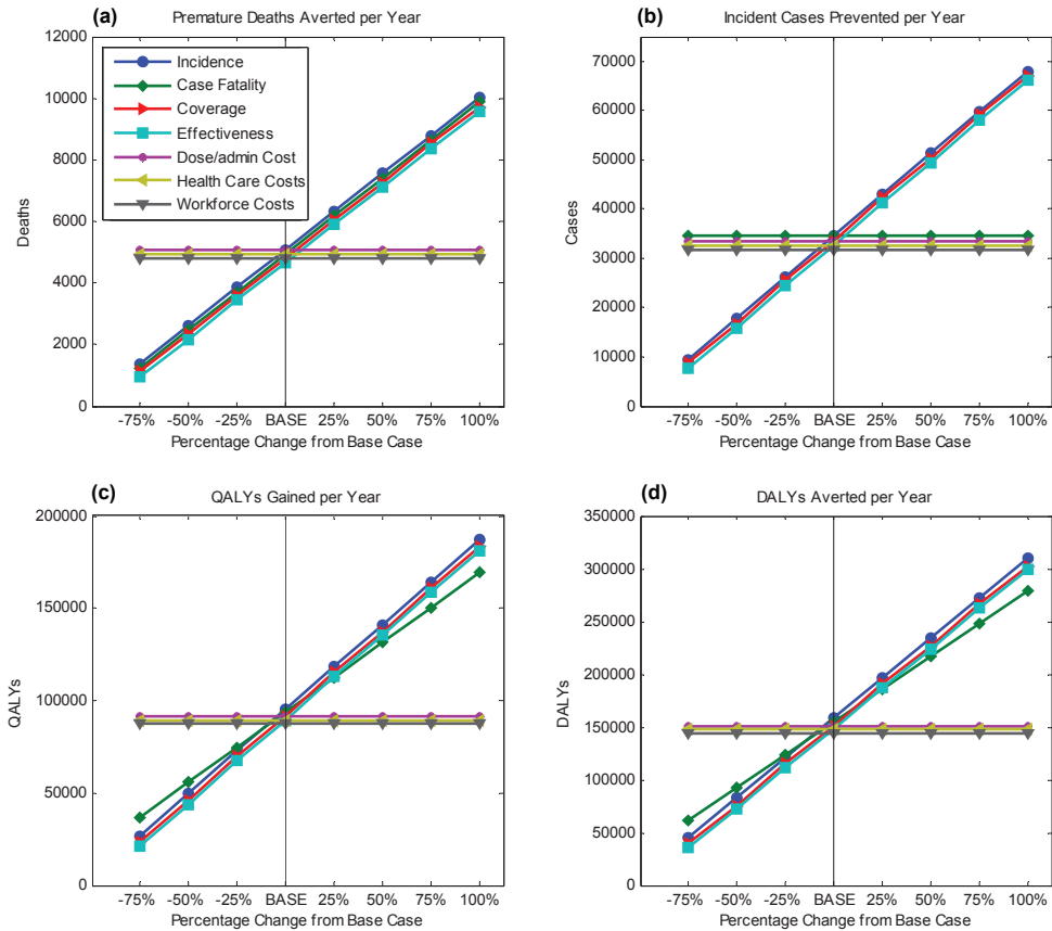
FIGURE D-4 Sensitivity analysis of the health-related attributes for a new tuberculosis vaccine for South Africa. The baseline scenarios from 2009 data were used to study the changes in 25 percent increments (-75% to 100%) for (a) premature deaths averted per year, (b) incident cases prevented per year, (c) QALYs gained per year, and (d) DALYs averted per year.
