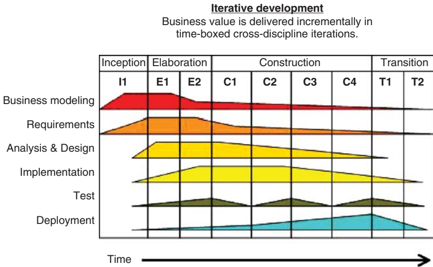
Figure 4.6 RUP SDLC 1
