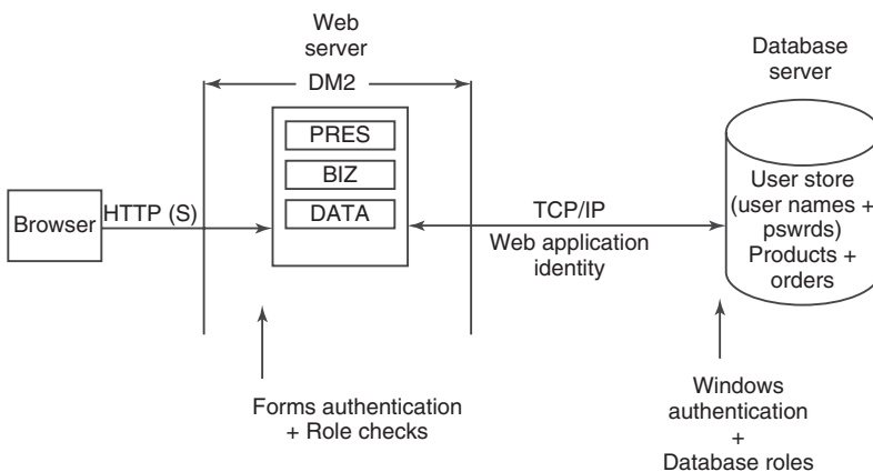
Figure 4.3 Sketched Architectural Diagram
