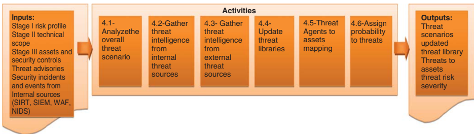
Figure 7.27 PASTA Risk-Centric Threat Modeling – Stage – IV (TA) Threat Analysis
