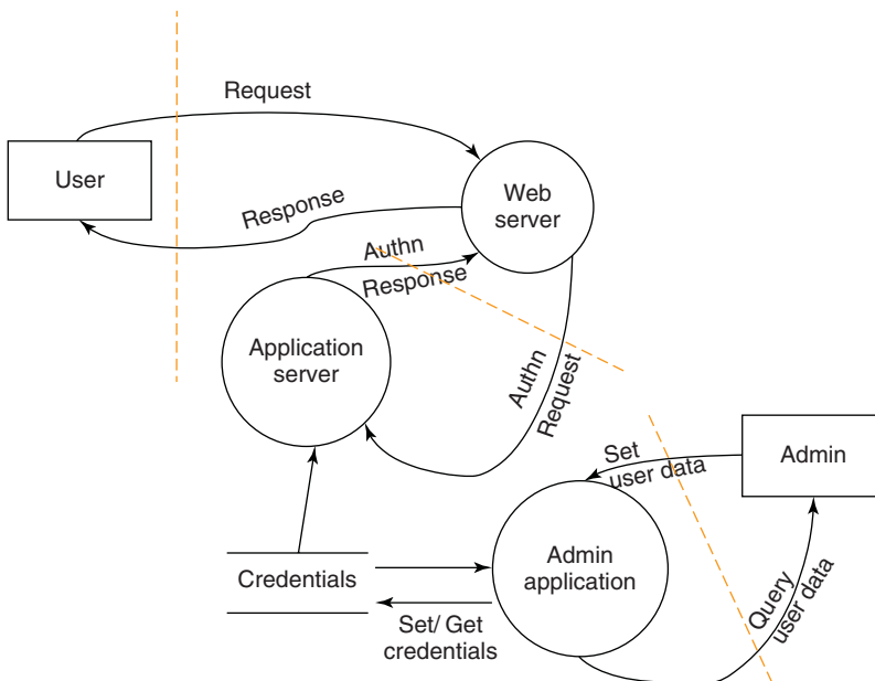
Figure 2.3 Example of Data Flow Diagram
