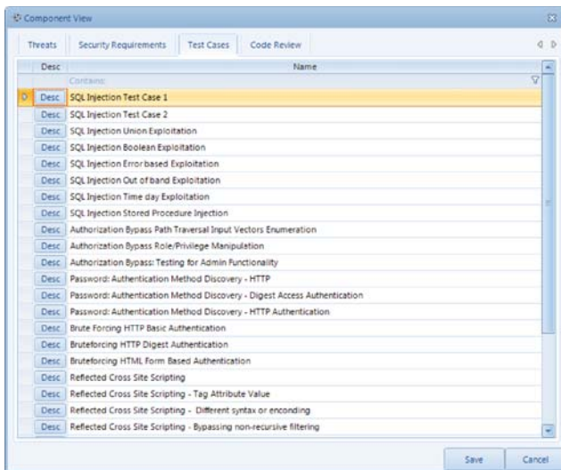
Figure 8.36 Threat-Level Security Test Cases
