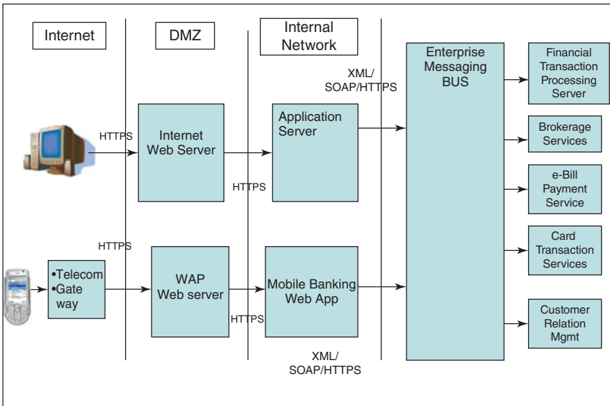
Figure 8.8 Architecture of Online Banking Application
