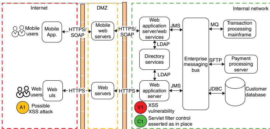
Figure 4.11 Generic Online Banking Application Threat Model
