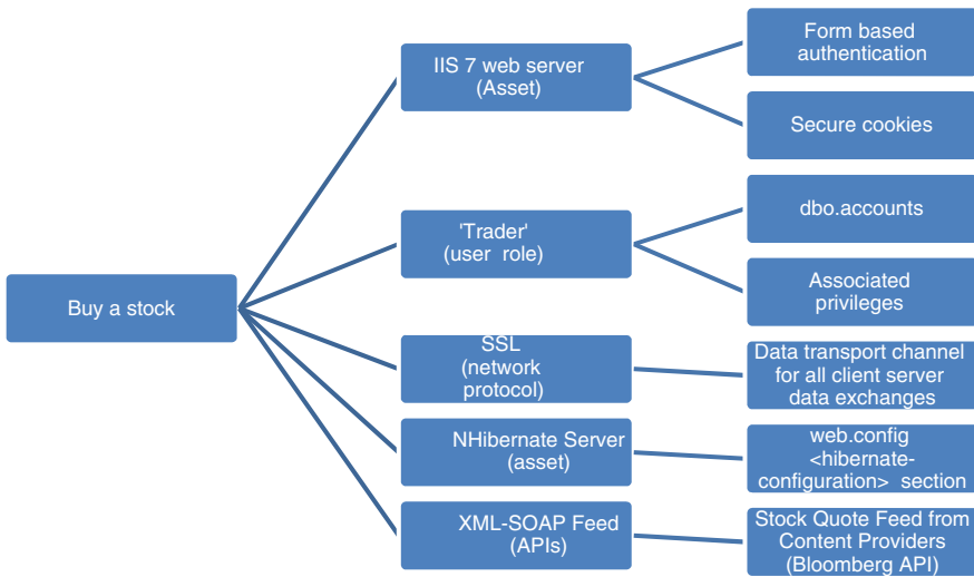
Figure 7.12 Use Case to Application Component Mapping
