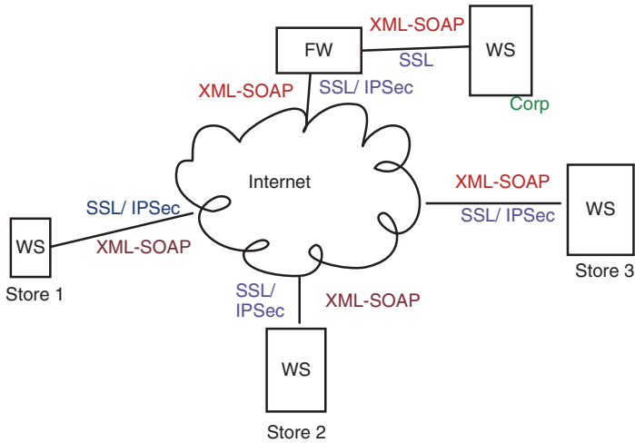
Figure 7.22 API from Stores Local Transaction Server with the Following Metadata
