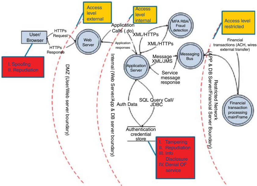
Figure 8.17 Threat Model Using STRIDE per Element
