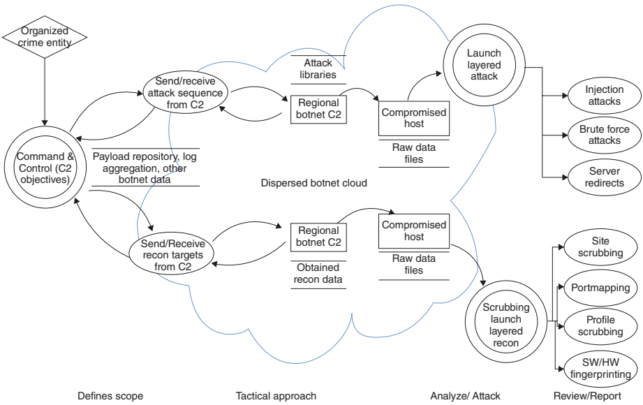
Figure 3.5 Security Centric DFD for Distributed Attacks
