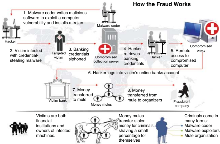
Figure 8.28 Anatomy of Account Takeover and Fraudulent Wire Transfer 4
