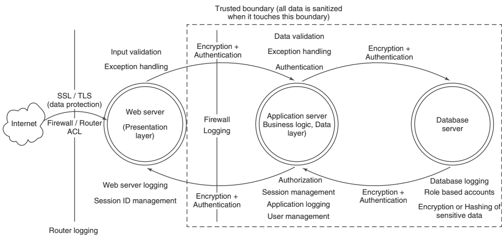
Figure 4.4 Data Flow Diagram
