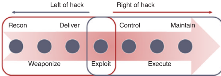
Figure 8.14 Example of Kill-Chain (Courtesy of MITRE corp) 2
