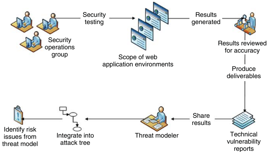
Figure 3.3 Process Overview of Vulnerability Assessment Integration to Threat Modeling
