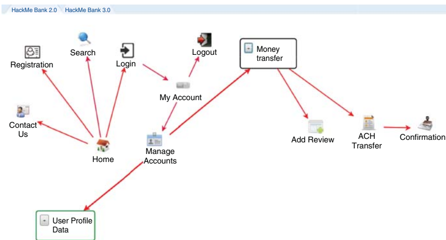
Figure 8.9 Component-Based Functional Use Cases of Online Web Application
