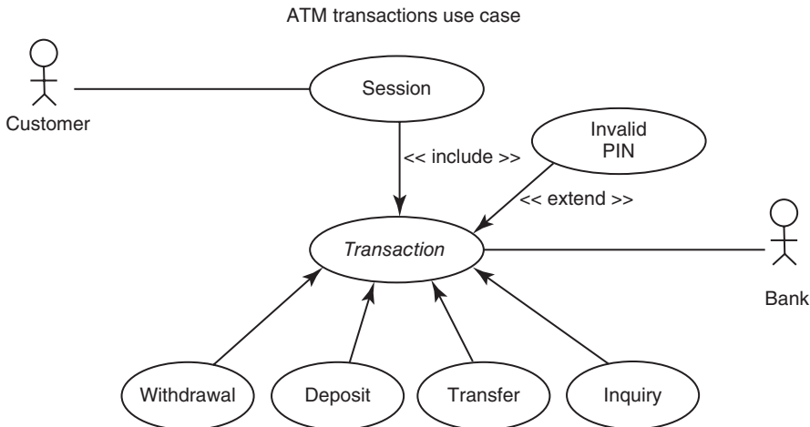
Figure 2.1 Example of Use Case Diagram 1
