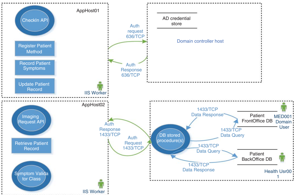
Figure 7.16 DFD Example Using Physical Boundaries for Organizing Components
