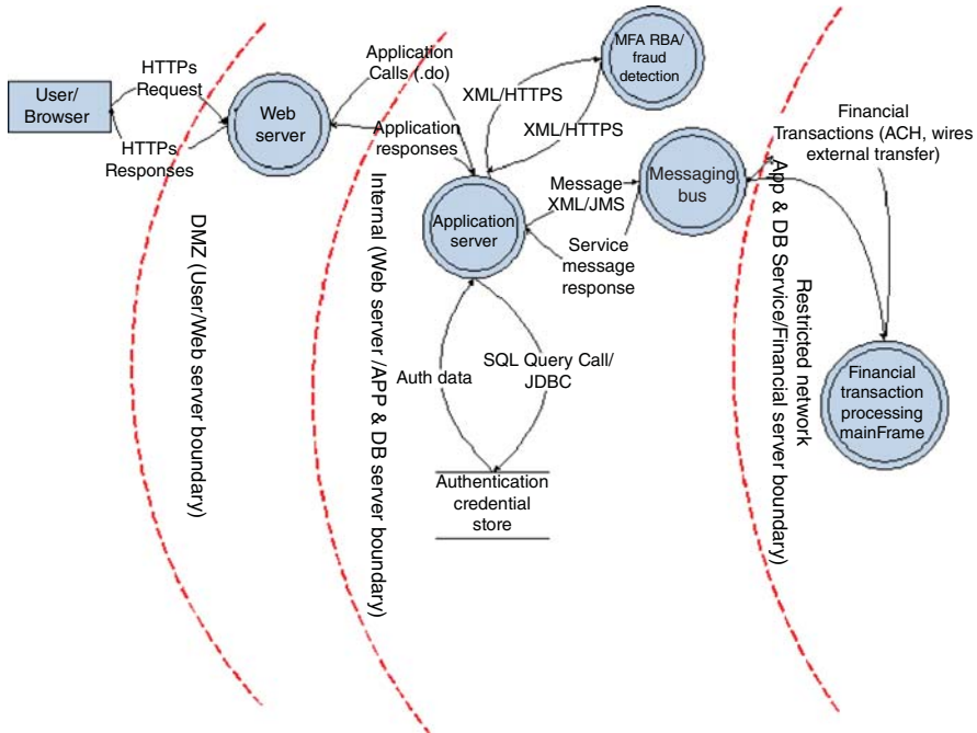
Figure 8.10 Data Flow Diagram for Online Banking Application
