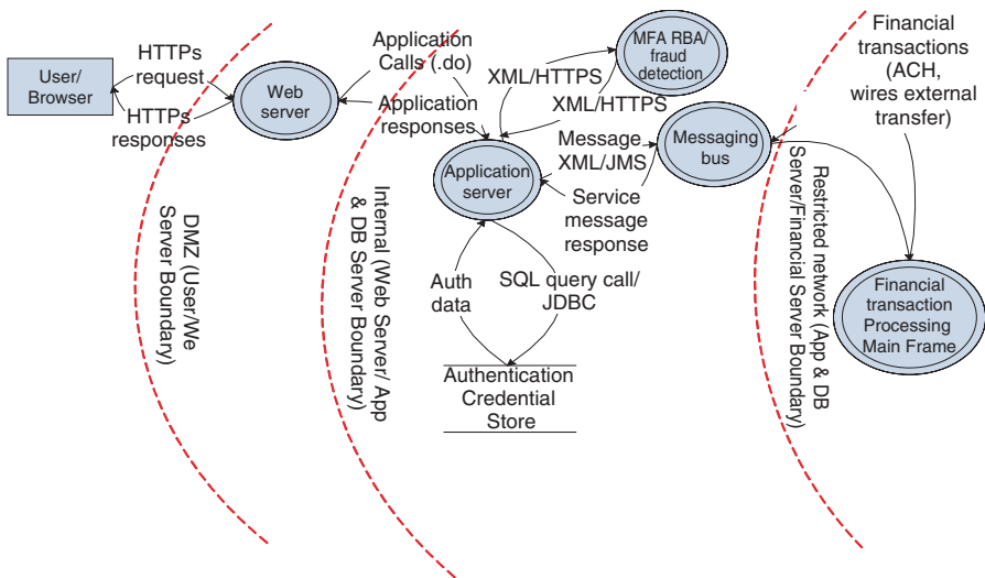
Figure 7.19 DFD Using Architectural Considerations for Component Grouping
