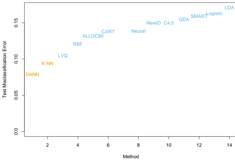
FIGURE 13.8. Test-error performance for a number of classifiers, as reported by the STATLOG project. The entry DANN is a variant of k -nearest neighbors, using an adaptive metric (Section 13.4.2).
