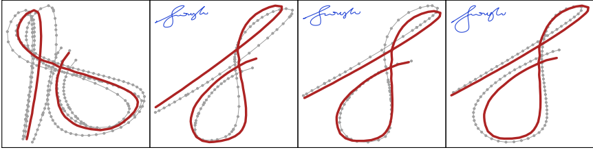
FIGURE 14.26. The Procrustes average of three versions of the leading S in Suresh's signatures. The left panel shows the preshape average, with each of the shapes \mathbf{X}_\ell^i in preshape space superimposed. The right three panels map the preshape \mathbf{M} separately to match each of the original S 's.
