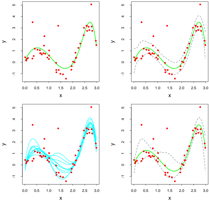
FIGURE 8.2. (Top left:) B -spline smooth of data. (Top right:) B -spline smooth plus and minus 1.96 \times standard error bands. (Bottom left:) Ten bootstrap replicates of the B -spline smooth. (Bottom right:) B -spline smooth with 95% standard error bands computed from the bootstrap distribution.
