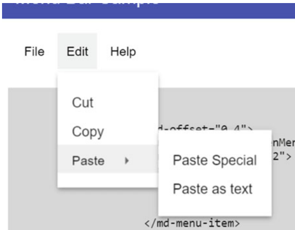
Figure 5-15. Nested menus
