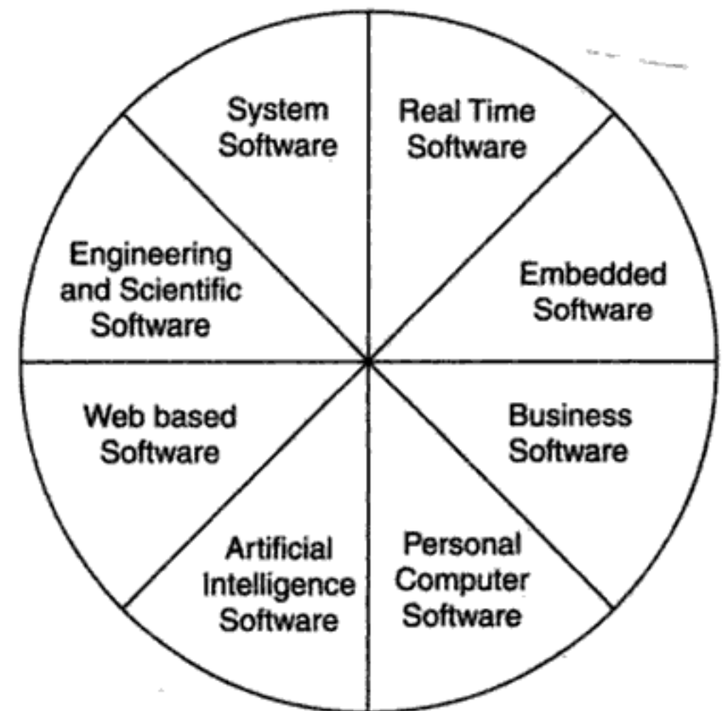
Fig. 1.7: Software applications.
