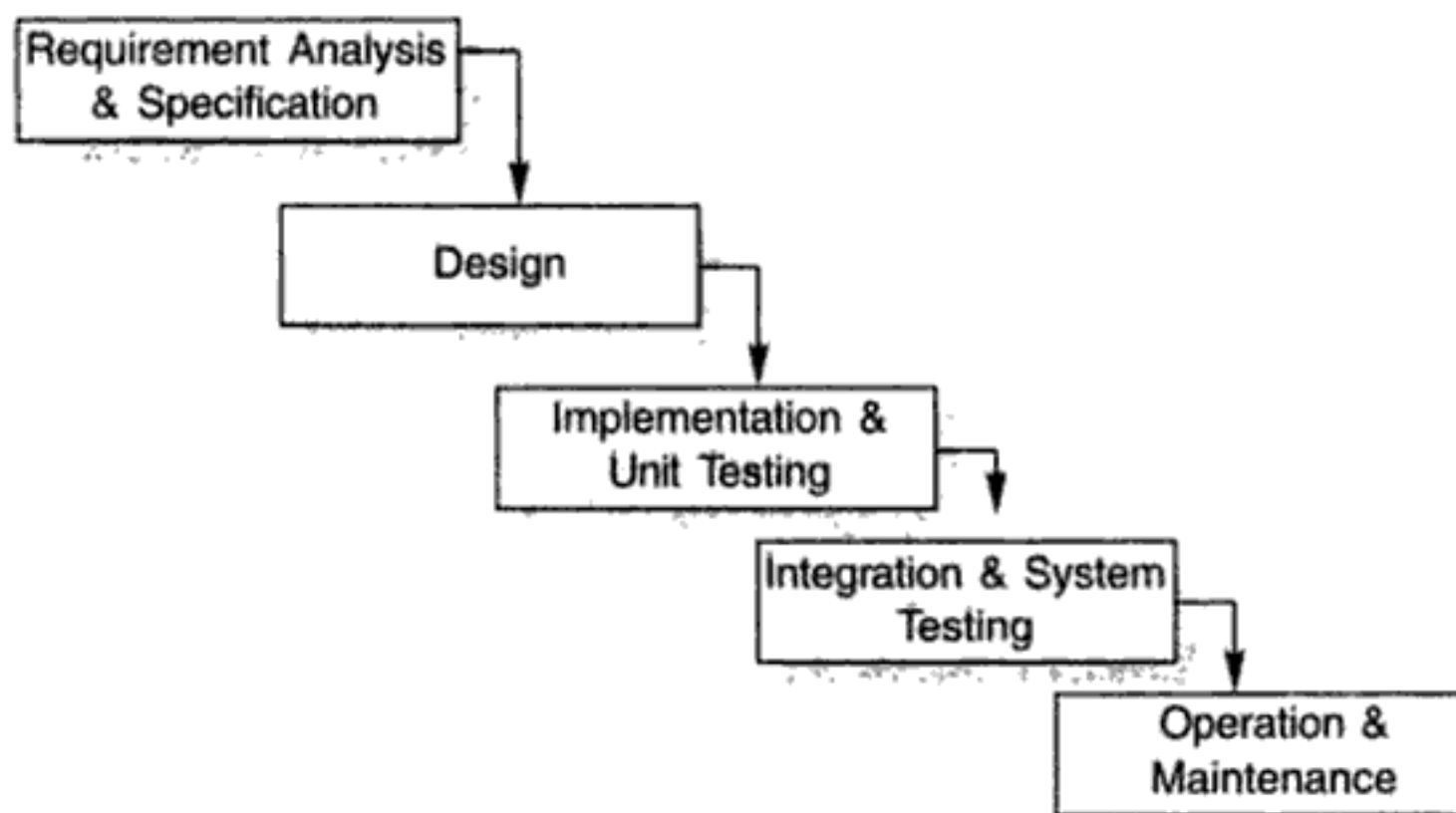
Fig. 2.2: Waterfall model
