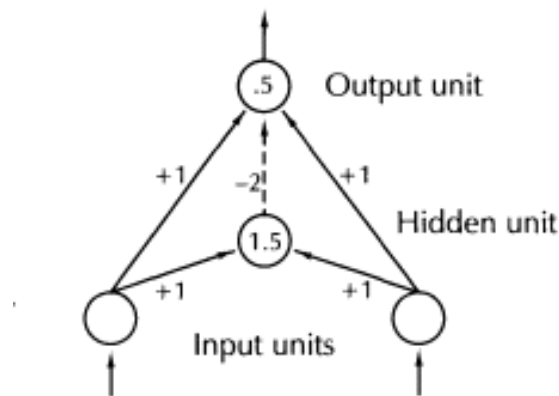
Figure 8.4: A simple XOR network with one hidden unit.
