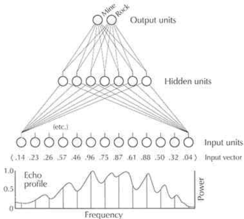
Figure 10.5: Perceptual recognition with a large network.
