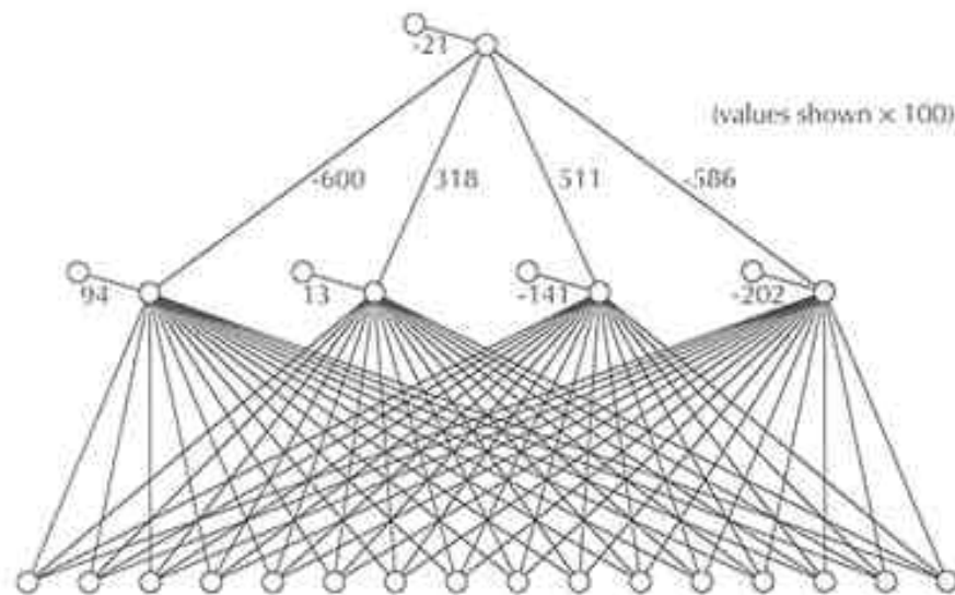
Figure 13.5: Network A again—now complete, but showing connection weights and biases only for hidden and output units.
