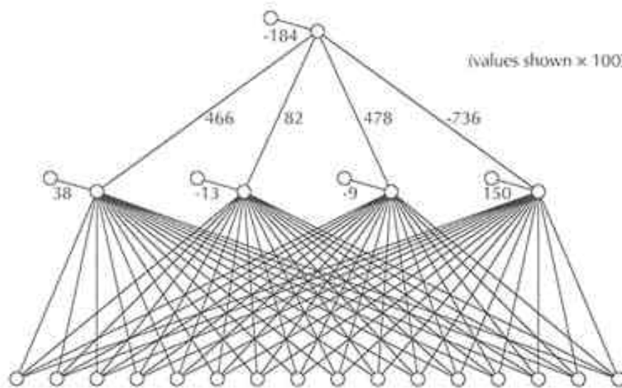
Figure 13.8: Network B, complete—showing weights and biases for hidden and output units.
