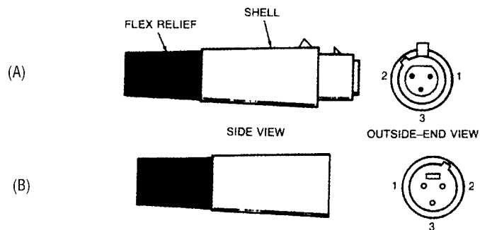
FIGURE 4.19 A 3-pin pro audio connector (XLR-type). (A) female; (B) male.
