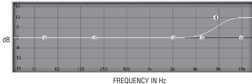
FIGURE 10.8 Shelving EQ at 7 kHz.
