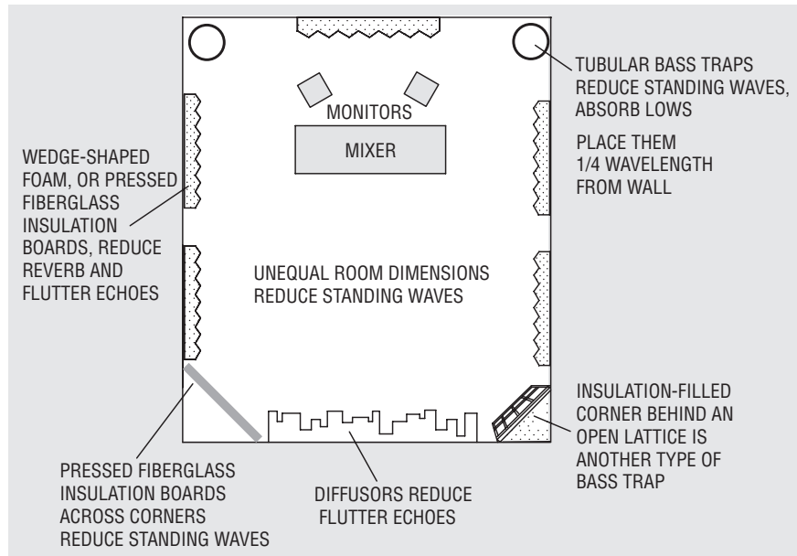
FIGURE 3.11 Acoustic treatments.
