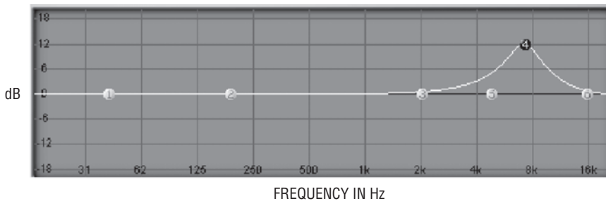
FIGURE 10.7 Peaking EQ at 7 kHz.
