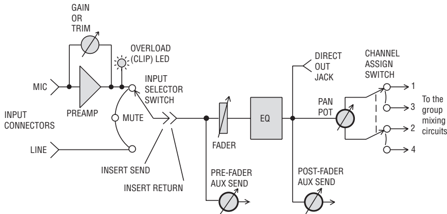
FIGURE 11.2 Signal flow through a typical input module.
