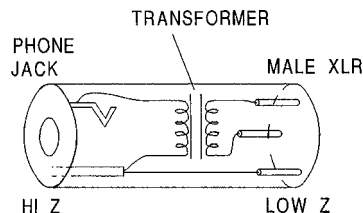
HI-TO-LOW IMPEDANCE MATCHING ADAPTER
