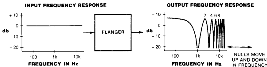
FIGURE 10.18 Flanging (or positive flanging).
