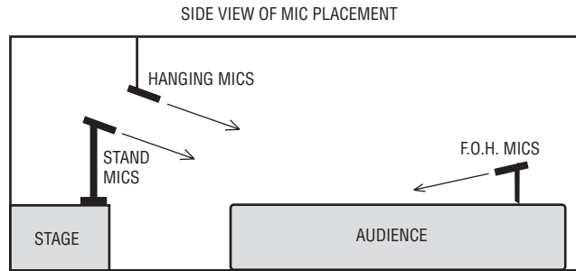
FIGURE 17.11 Some audience miking techniques.
