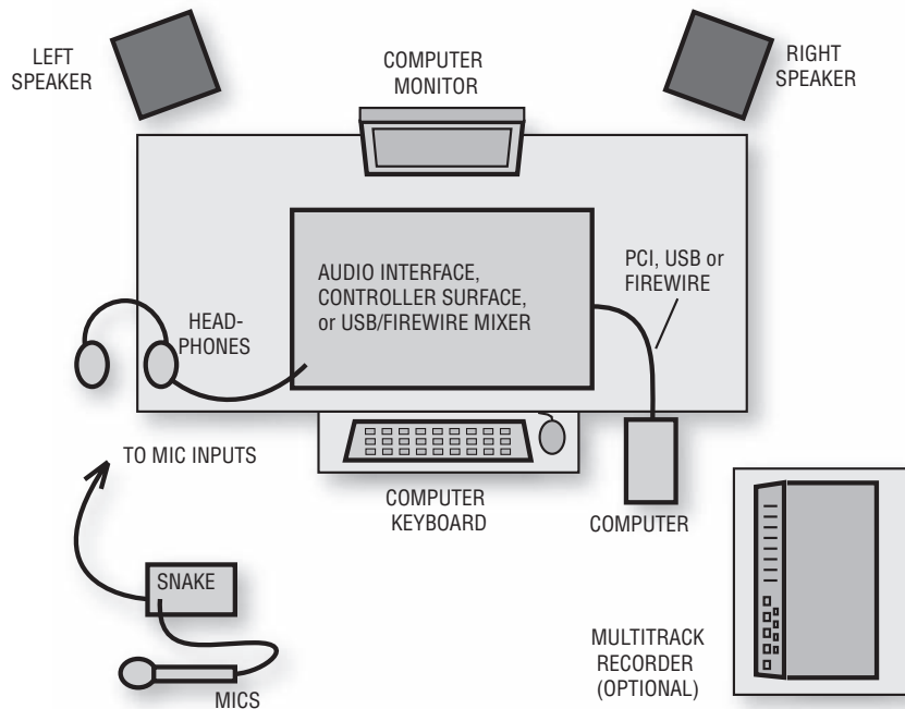
FIGURE 4.27 Typical layout of a DAW recording studio.
