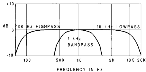
FIGURE 10.9 Lowpass, highpass, and bandpass filters.
