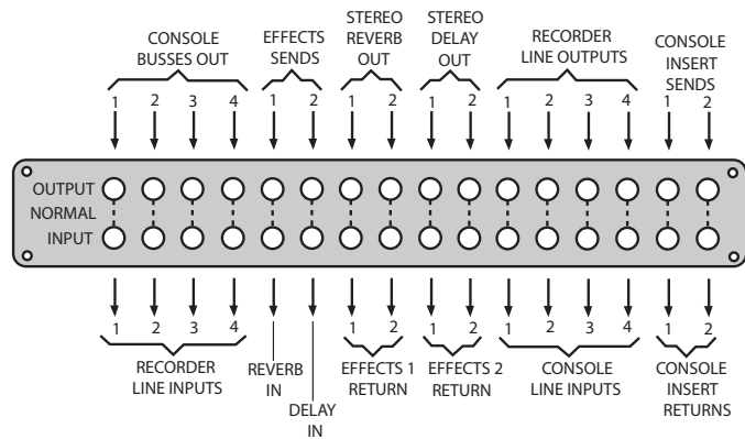
Figure 4.23 Some typical patch-bay assignments.
