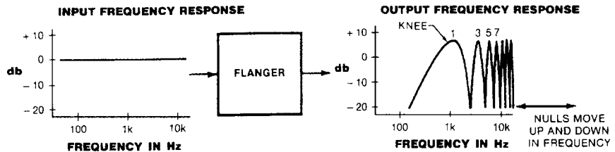
FIGURE 10.19 Negative flanging.
