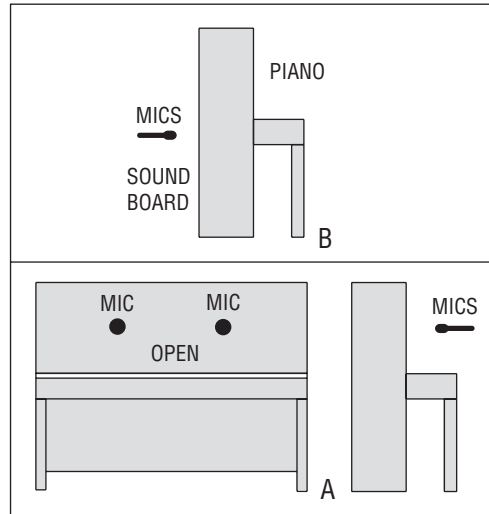
FIGURE 8.16 Some mic techniques for upright piano.
