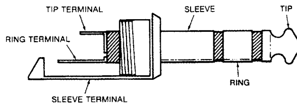
FIGURE 4.20 A stereo (TRS) phone plug.
