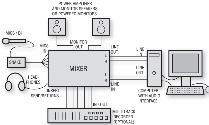
FIGURE 4.24 Typical connections for recording-studio equipment.
