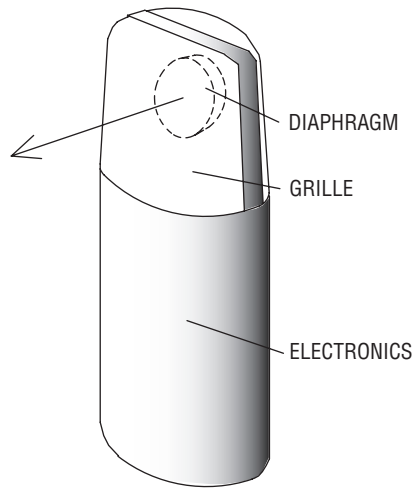
FIGURE 6.6 A typical multi-pattern mic that is side-addressed.
