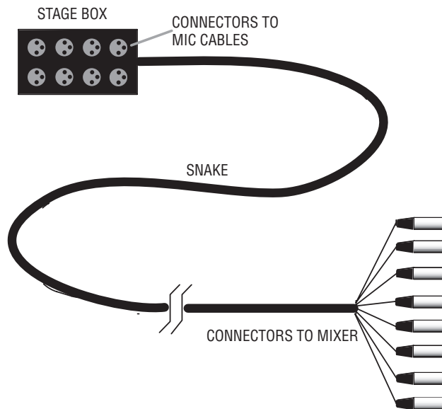
FIGURE 4.21 A stage box and snake.
