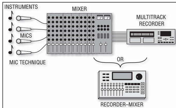
FIGURE 2.3 The recording chain for multitrack recording.
