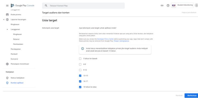
Gambar 4. 37 penargetan audiens
