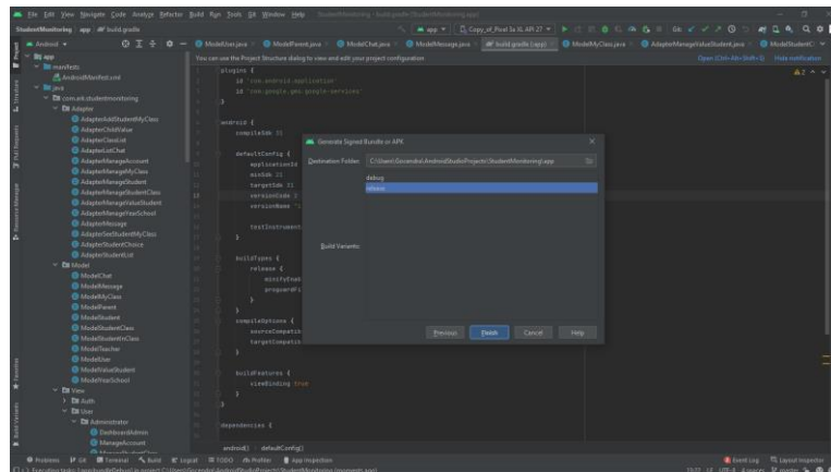
Gambar 4. 26 release
