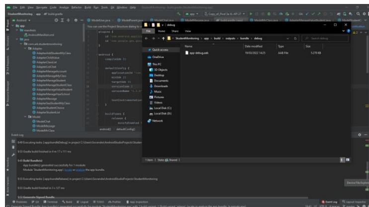
Gambar 4. 27 generate build
