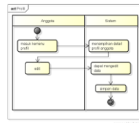
Gambar 4.4 Activity Diagram Profil
