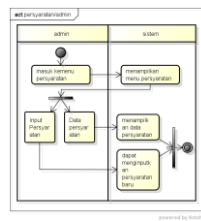
Gambar 4.12 Activity Diagram Input Persyaratan
