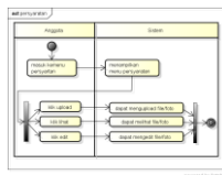
Gambar 4.6 Activity Diagram Persyaratan
