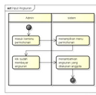
Gambar 4.11 Activity Diagram Input Angsuran
