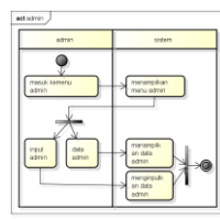
Gambar 4.13 Activity Diagram Input Admin
