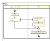
Gambar 4.3 Activity Diagram Login
