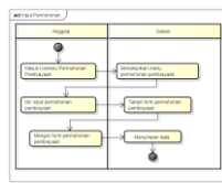
Gambar 4.5 Activity Diagram Input Permohonan
