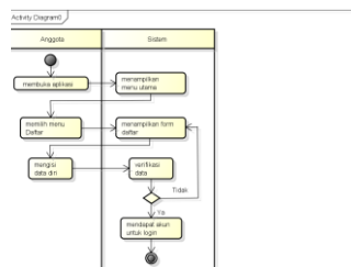
Gambar 4.2 Activity Diagram Daftar
