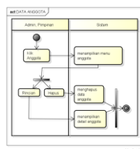
Gambar 4.9 Activity Diagram View Data Anggota
