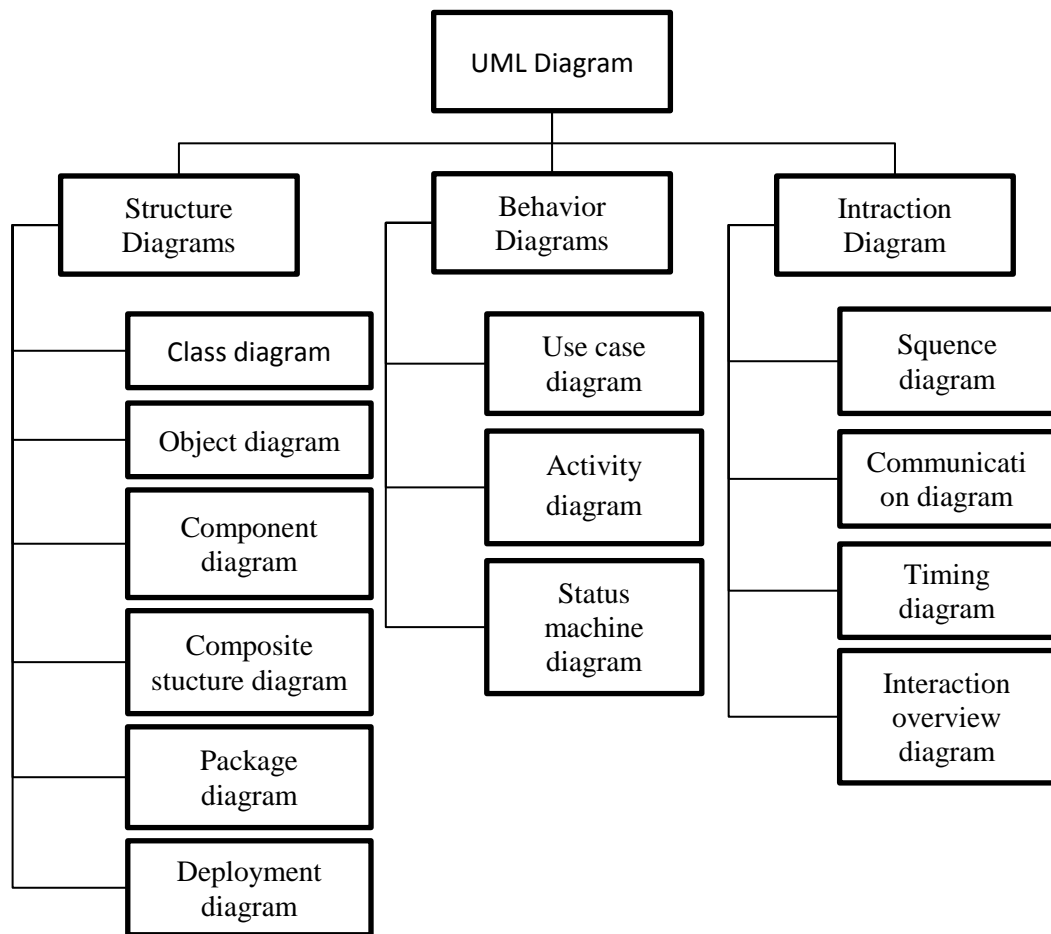
Gambar 2.2 Diagram UML
