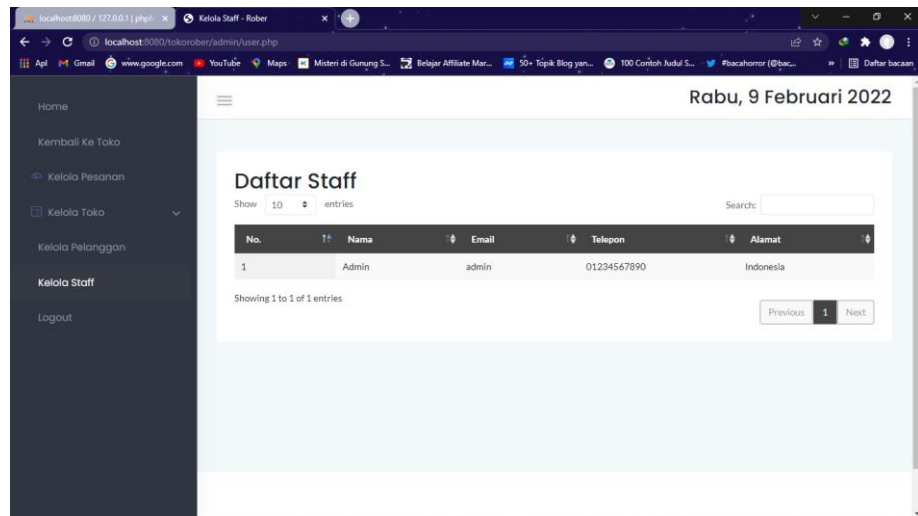
Gambar 4.11 Tampilan Staff
