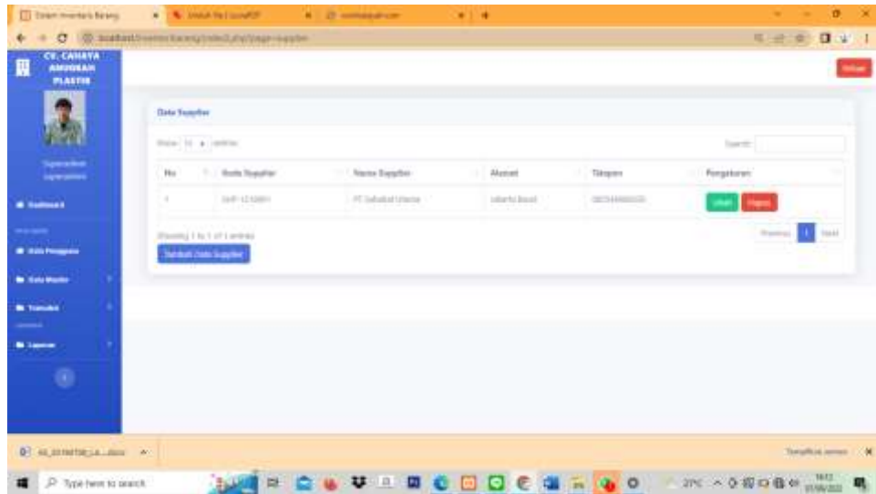
Gambar 3.21 Tampilan Supplier
