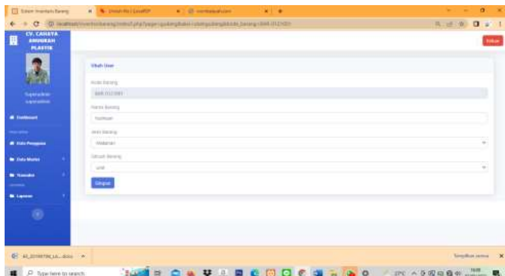
Gambar 3.17 Edit Barang
