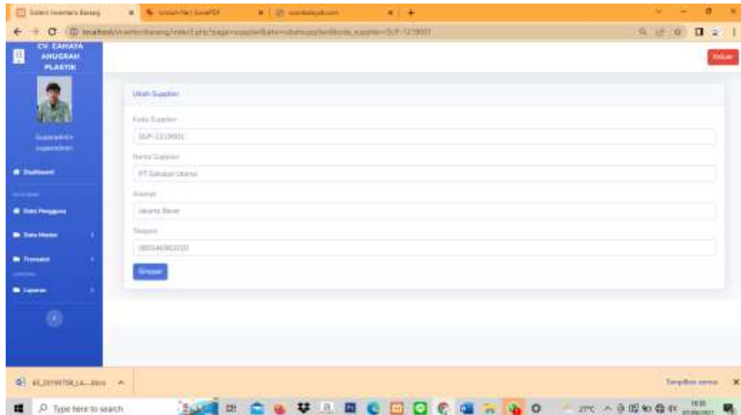
Gambar 3.23 Edit Supplier
