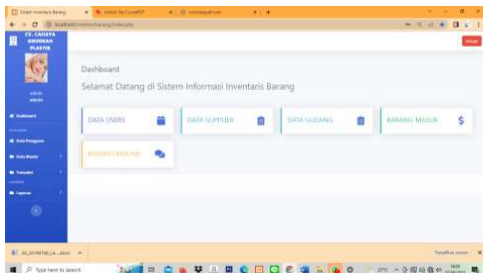
Gambar 3.11 Dashboard Admin
