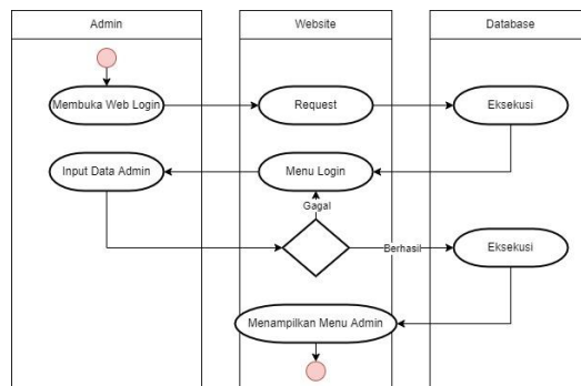
Gambar 4. Activity Diagram Admin
